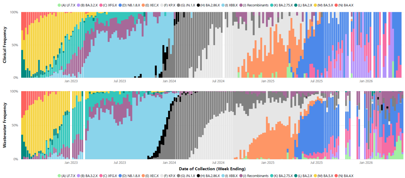
Figure 18. Distribution of SARS-CoV-2 variants in clinical samples (top) and metropolitan wastewater catchments (bottom), 3 July 2022 to 17 May 2026
